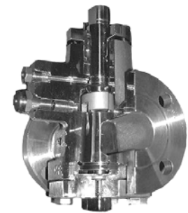
Metal Seated Plug Valve, Lubricated, RF FIG 125, 325, 625, 1525
