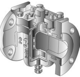
3Z Lined Plug Valve
