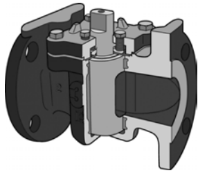
3Z Sleeved Plug Valve
