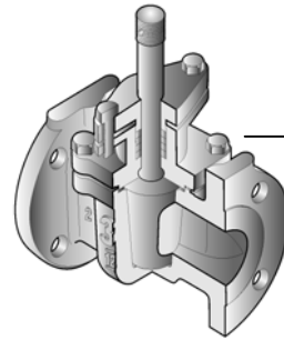
3Z Metal Seated Plug Valve Non-Lubricated
