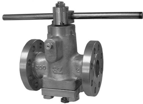
3Z Hydrofluoric Acid Service Valve Port Plug Valve FIG 120HF, 320HF, 620HF
