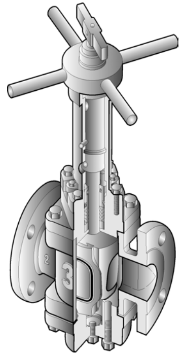
3Z Double Block & Bleed Plug Valve, Non-Lubricated,
